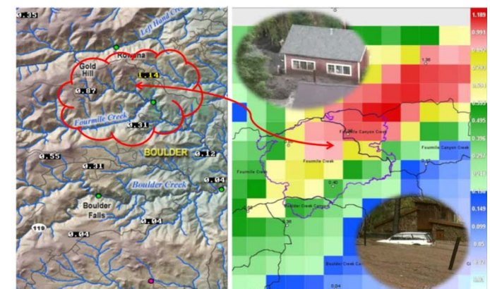
Rainfall totals from the ALERT system and Radar estimates of rainfall that caused the flash flood of July 13, 2011
